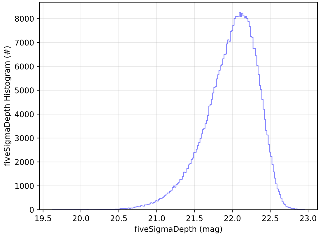
ddf_acor_sf10_lsf30_lsr10_v3.4_10yrs All sky y band: fiveSigmaDepth Histogram
