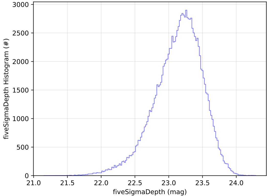
ddf_acor_sf10_lsf30_lsr10_v3.4_10yrs All sky u band: fiveSigmaDepth Histogram
