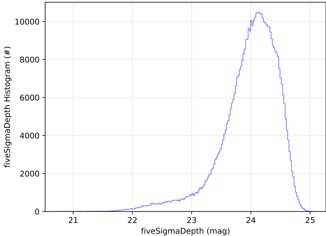
ddf_acor_sf10_lsf30_lsr10_v3.4_10yrs All sky r band: fiveSigmaDepth Histogram
