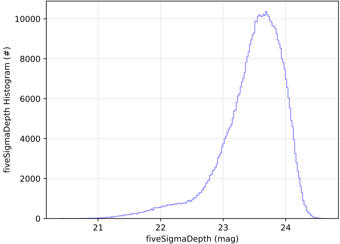
ddf_acor_sf10_lsf30_lsr10_v3.4_10yrs All sky i band: fiveSigmaDepth Histogram
