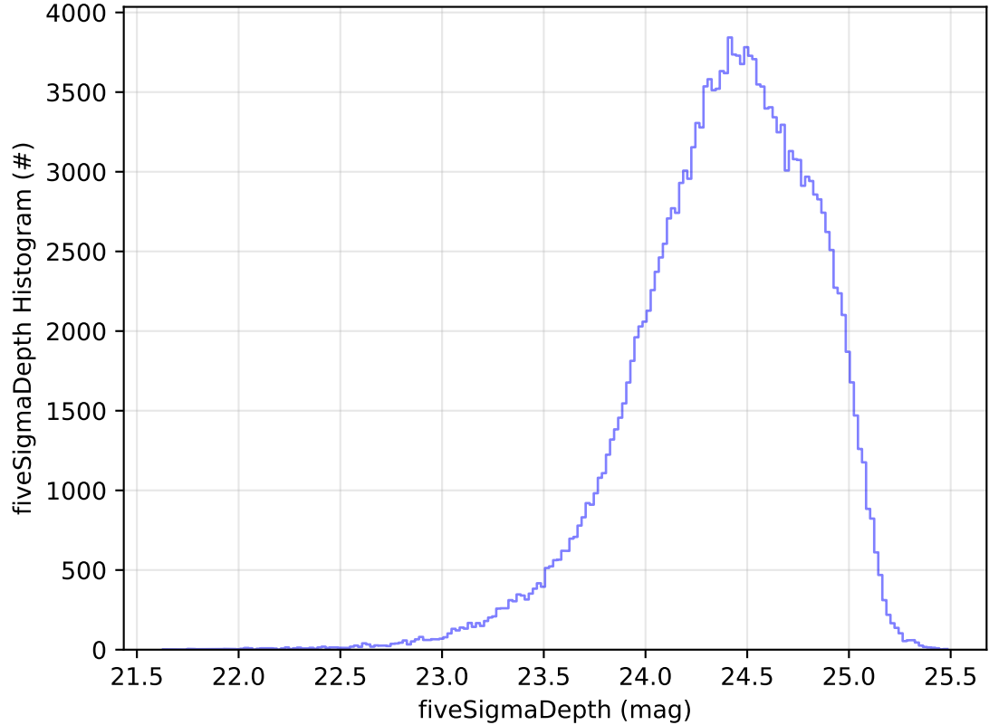
ddf_acor_sf10_lsf30_lsr10_v3.4_10yrs All sky g band: fiveSigmaDepth Histogram
