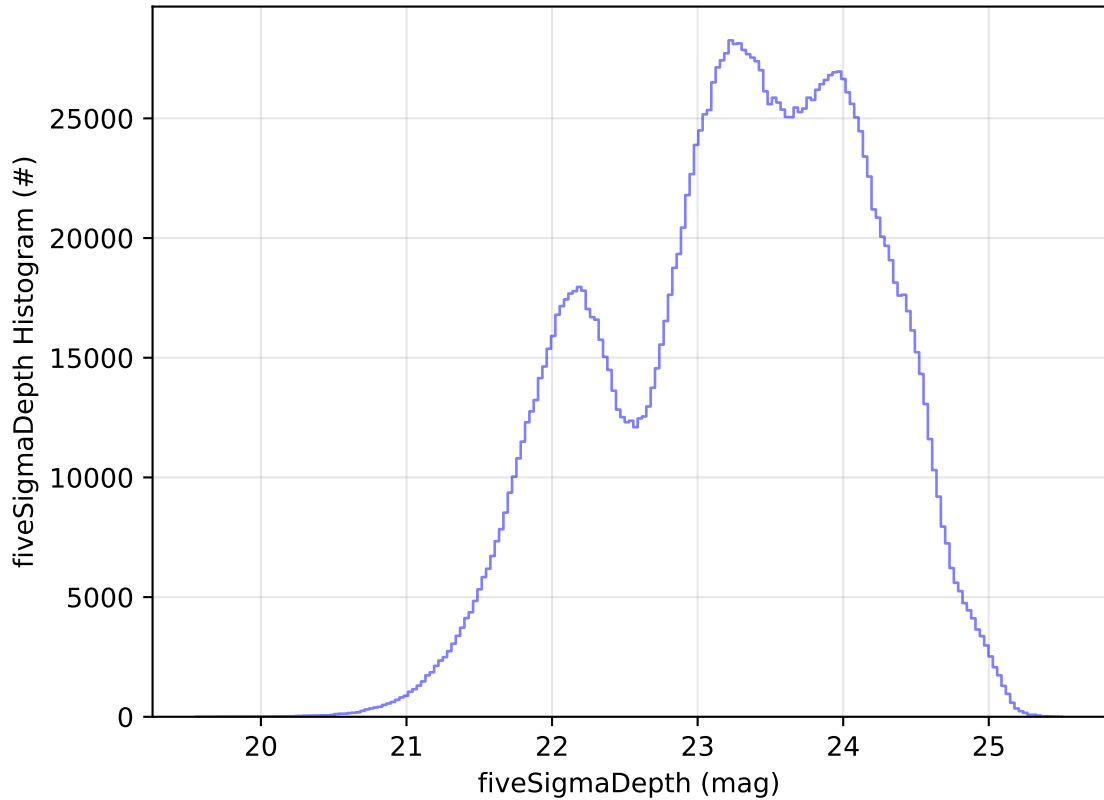
ddf_acor_sf10_lsf30_lsr10_v3.4_10yrs All sky all bands: fiveSigmaDepth Histogram
