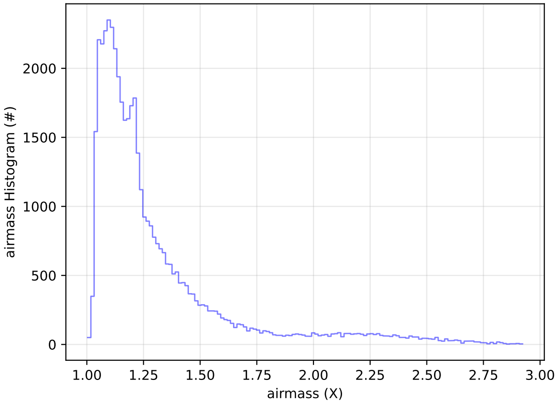
ddf_acor_sf10_lsf30_lsr10_v3.4_10yrs Yr 1 z band: airmass Histogram
