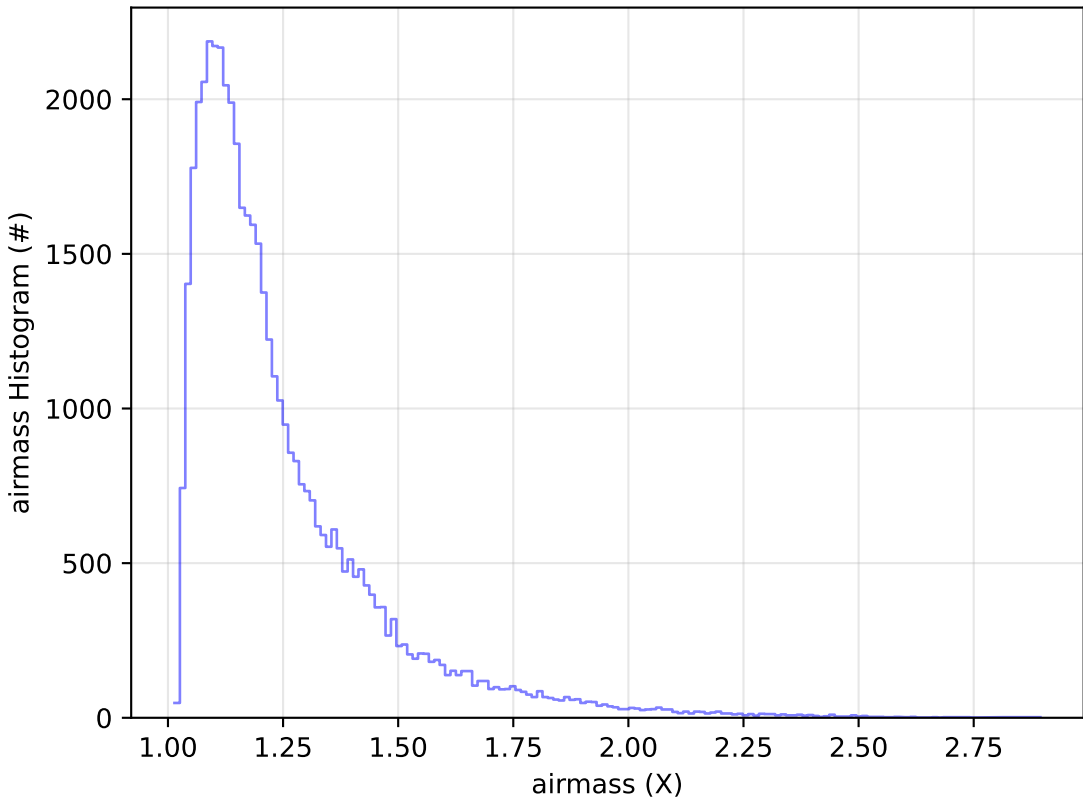
ddf_acor_sf10_lsf30_lsr10_v3.4_10yrs Yr 1 y band: airmass Histogram
