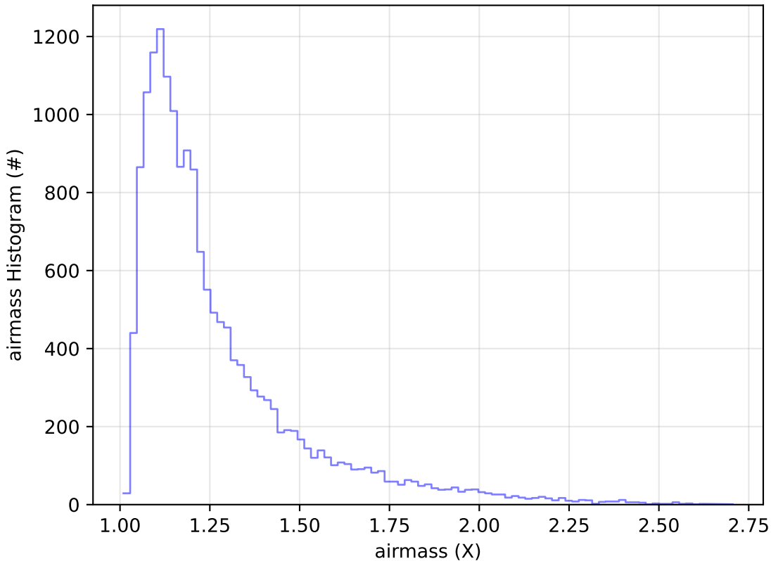
ddf_acor_sf10_lsf30_lsr10_v3.4_10yrs Yr 1 u band: airmass Histogram
