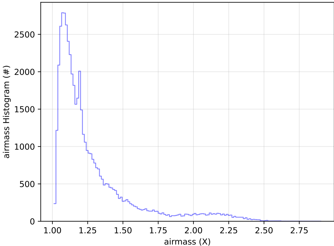
ddf_acor_sf10_lsf30_lsr10_v3.4_10yrs Yr 1 r band: airmass Histogram
