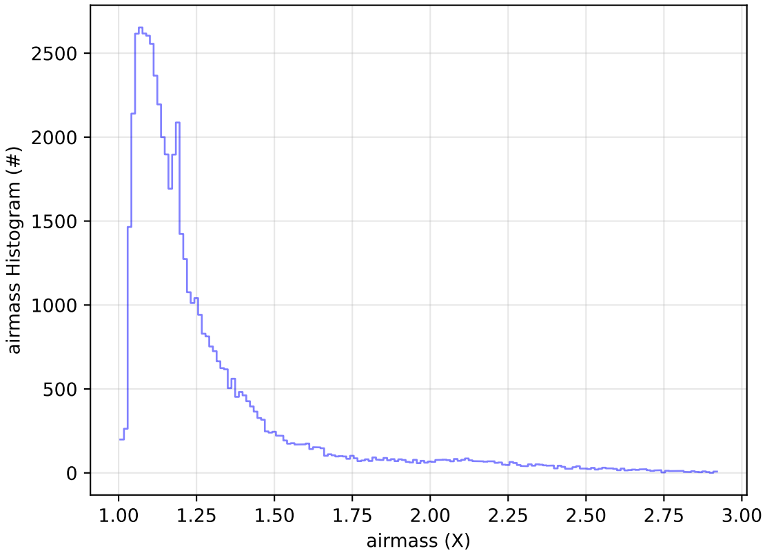
ddf_acor_sf10_lsf30_lsr10_v3.4_10yrs Yr 1 i band: airmass Histogram
