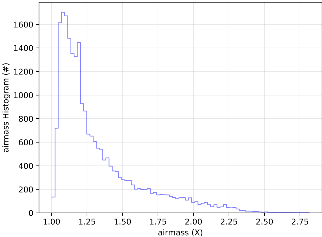
ddf_acor_sf10_lsf30_lsr10_v3.4_10yrs Yr 1 g band: airmass Histogram
