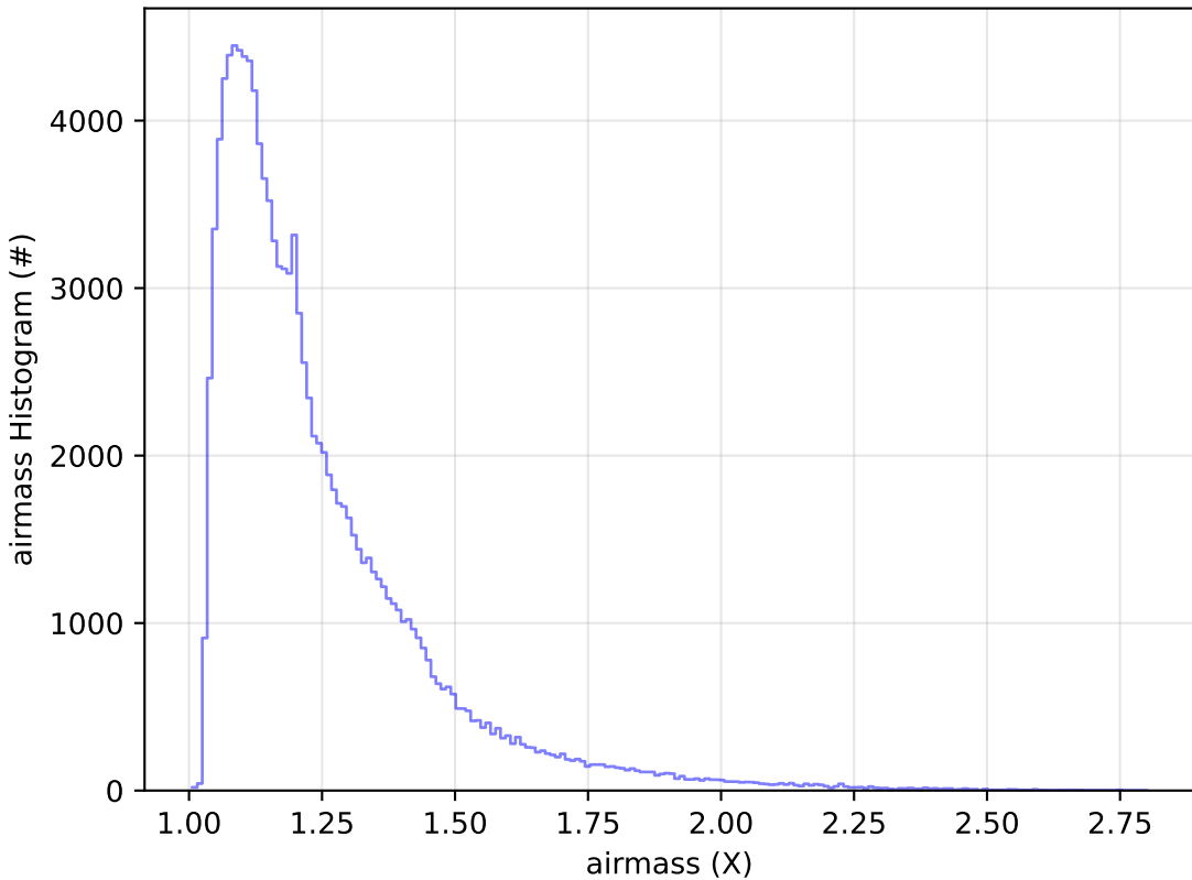
ddf_acor_sf10_lsf30_lsr10_v3.4_10yrs WFD u band: airmass Histogram
