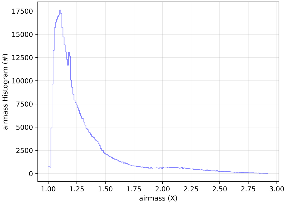
ddf_acor_sf10_lsf30_lsr10_v3.4_10yrs WFD i band: airmass Histogram
