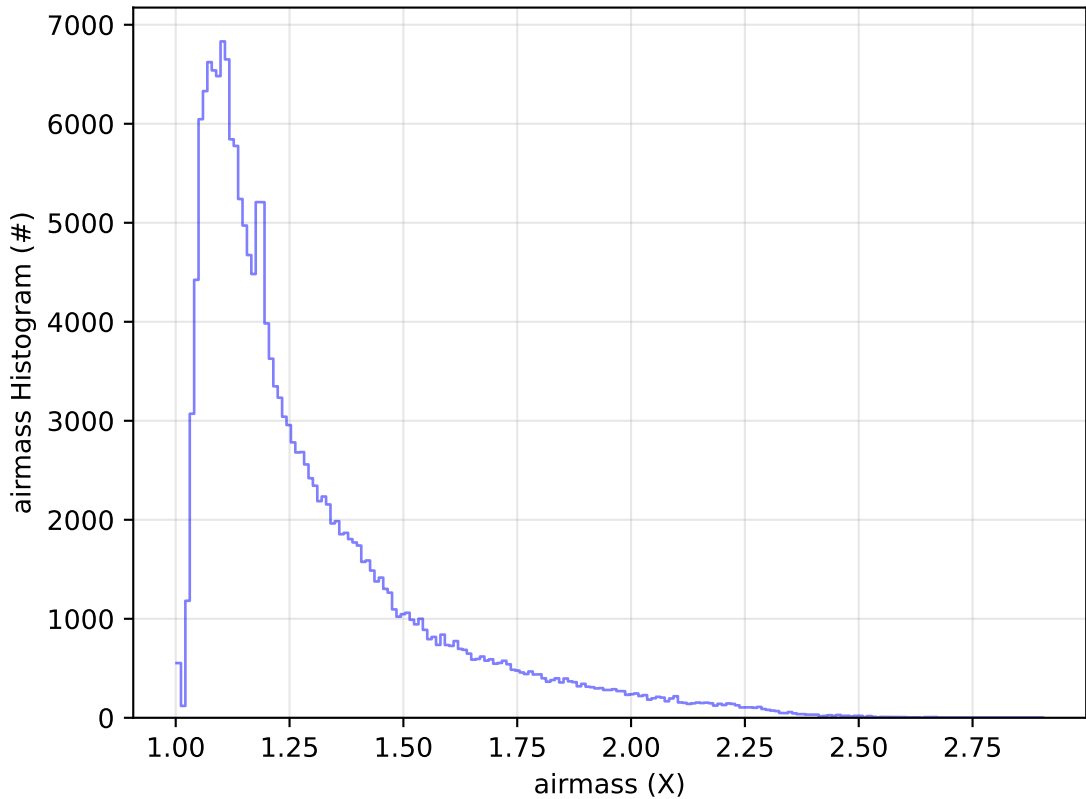
ddf_acor_sf10_lsf30_lsr10_v3.4_10yrs WFD g band: airmass Histogram
