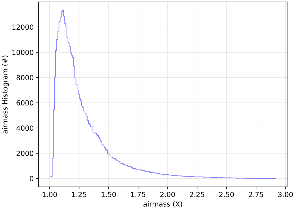
ddf_acor_sf10_lsf30_lsr10_v3.4_10yrs All sky y band: airmass Histogram
