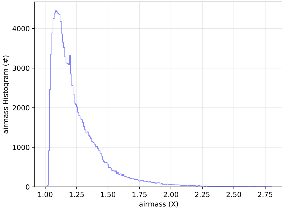
ddf_acor_sf10_lsf30_lsr10_v3.4_10yrs All sky u band: airmass Histogram
