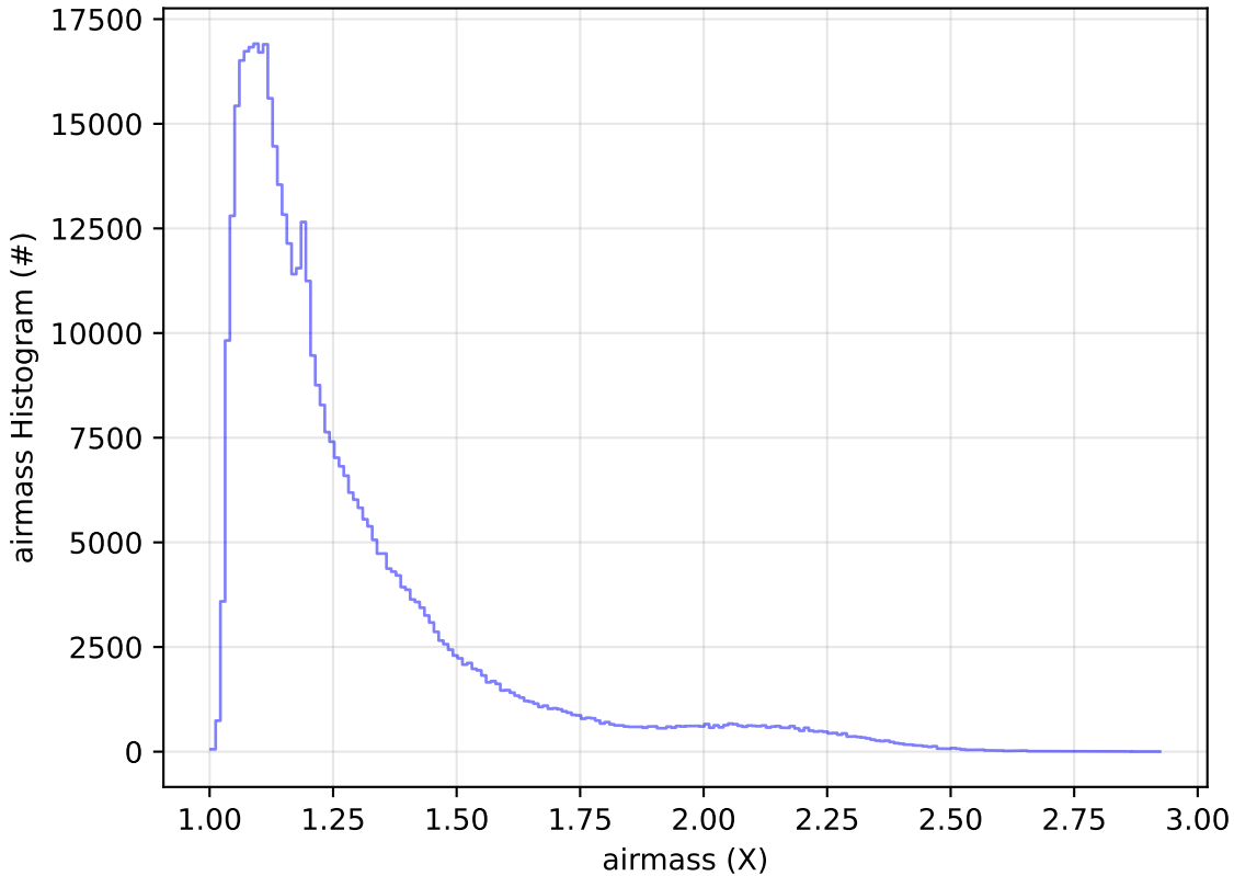
ddf_acor_sf10_lsf30_lsr10_v3.4_10yrs All sky r band: airmass Histogram
