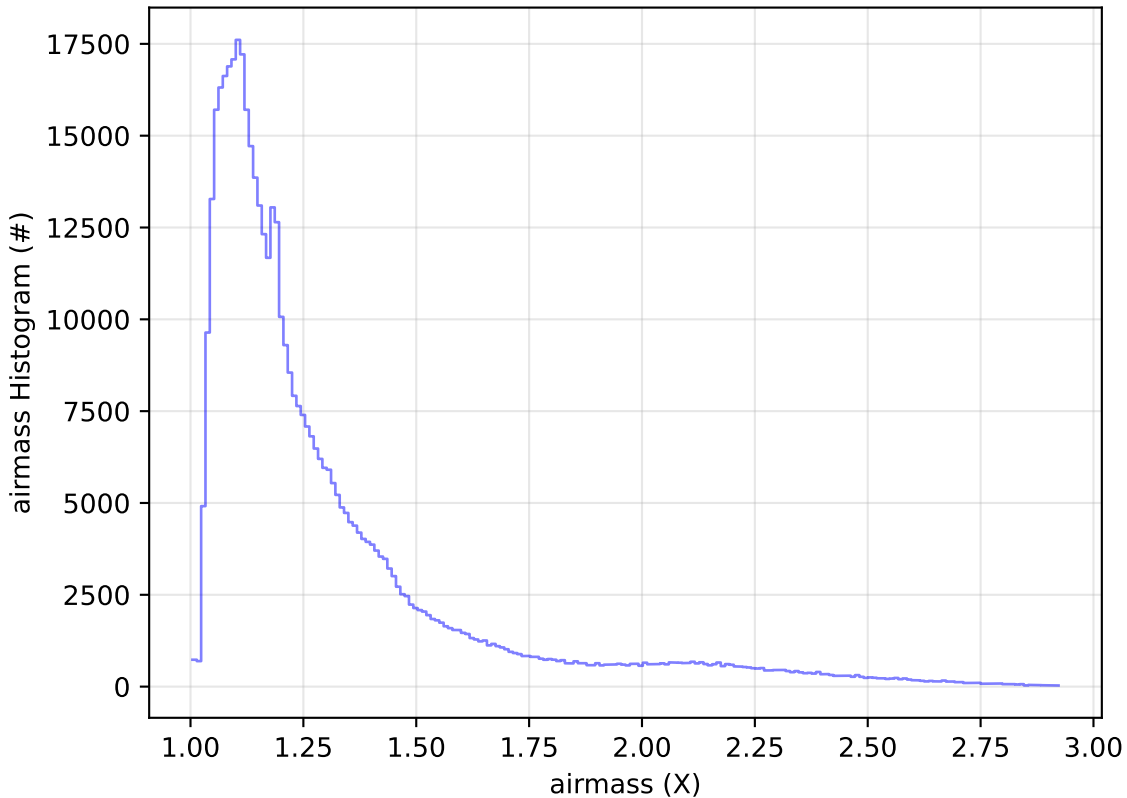
ddf_acor_sf10_lsf30_lsr10_v3.4_10yrs All sky i band: airmass Histogram
