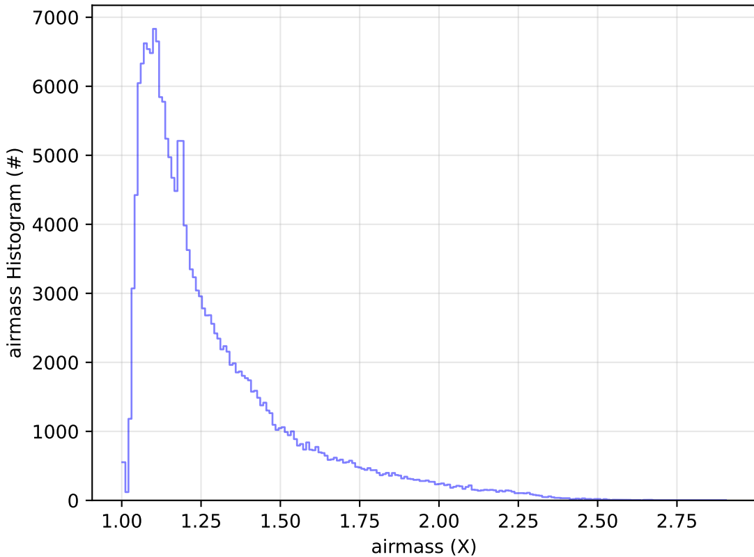
ddf_acor_sf10_lsf30_lsr10_v3.4_10yrs All sky g band: airmass Histogram
