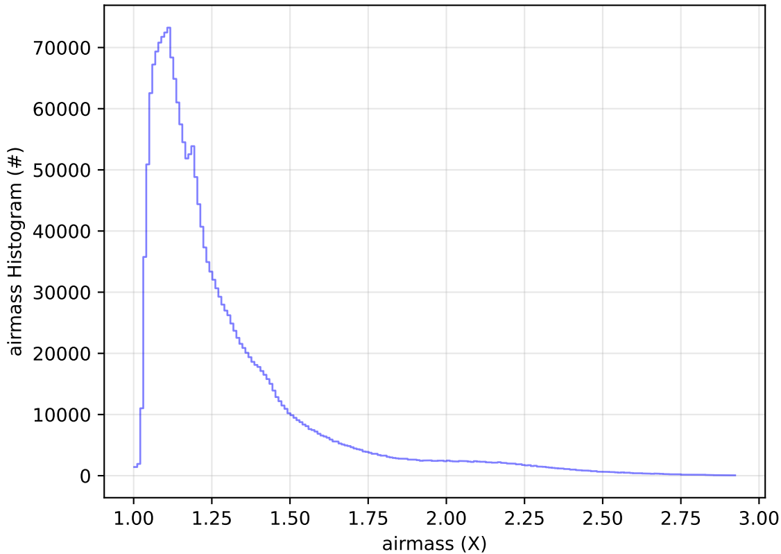
ddf_acor_sf10_lsf30_lsr10_v3.4_10yrs All sky all bands: airmass Histogram
