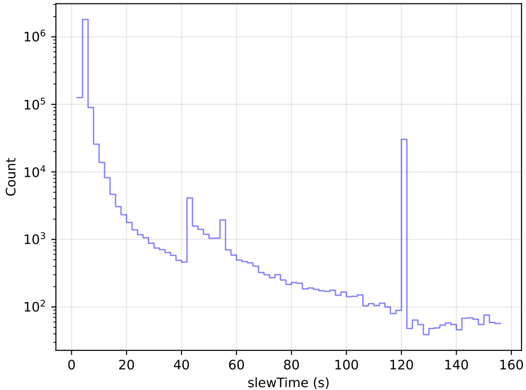
ddf_acor_sf10_lsf30_lsr10_v3.4_10yrs All visits: Slew Time Histogram
