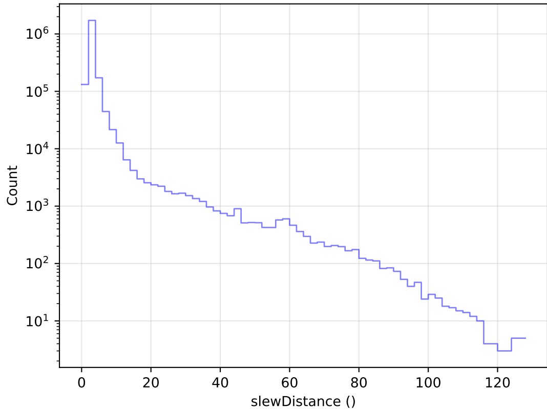
ddf_acor_sf10_lsf30_lsr10_v3.4_10yrs All visits: Slew Distance Histogram
