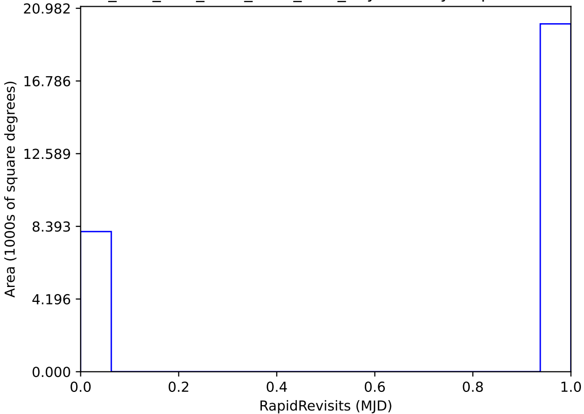
ddf_acor_sf10_lsf30_lsr10_v3.4_10yrs All sky: RapidRevisits
