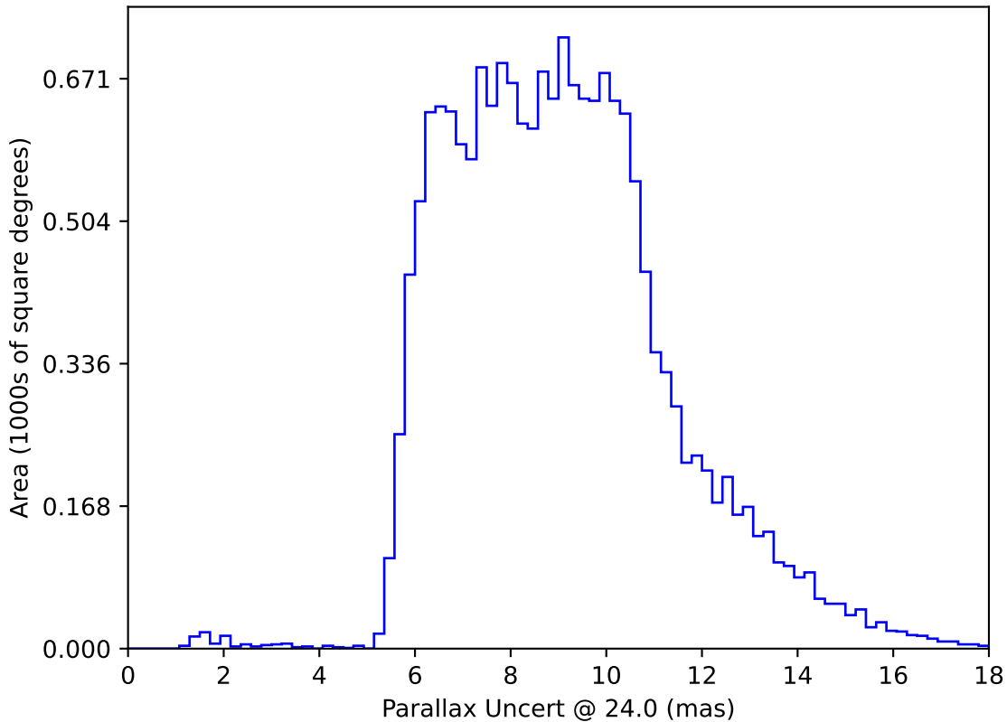
ddf_acor_sf10_lsf30_lsr10_v3.4_10yrs WFD: Parallax Uncert @ 24.0
