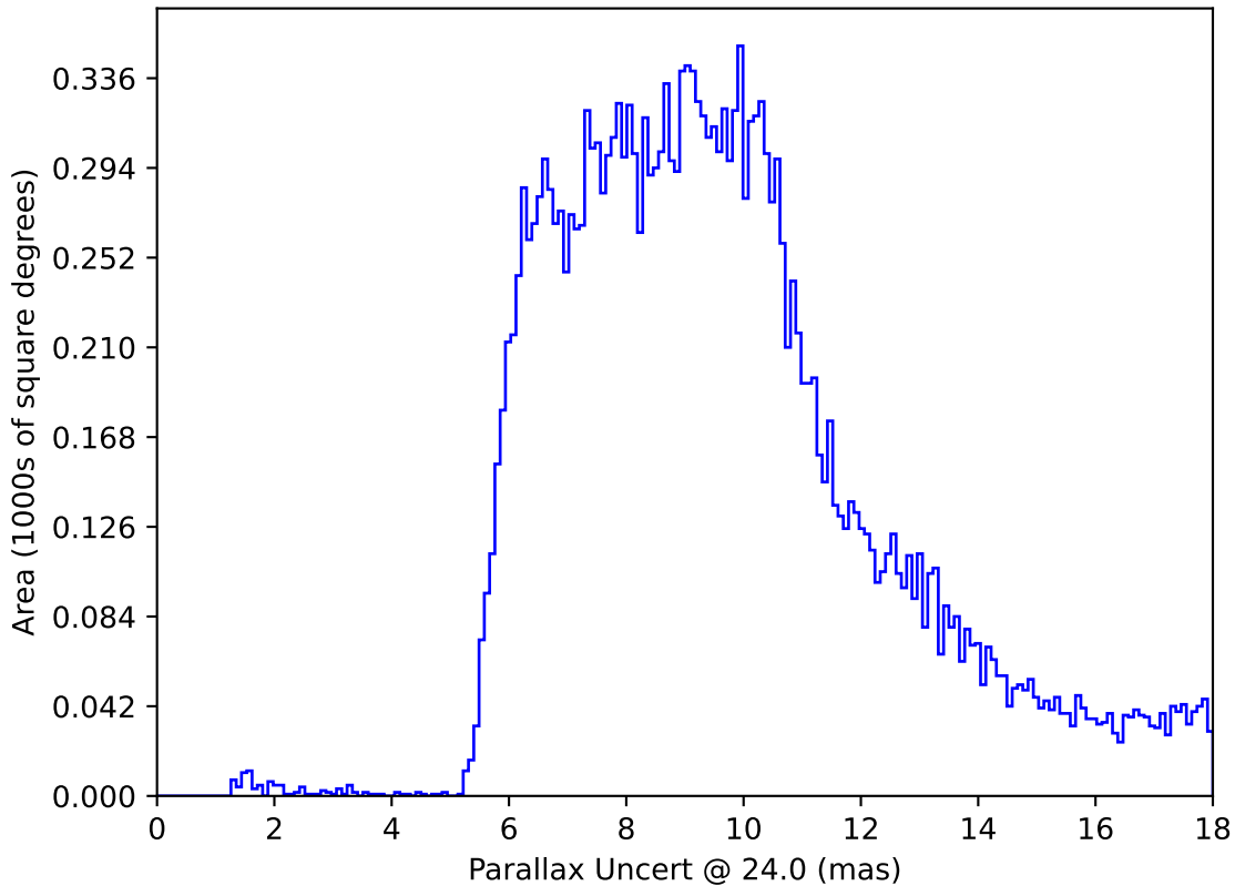
ddf_acor_sf10_lsf30_lsr10_v3.4_10yrs All sky: Parallax Uncert @ 24.0
