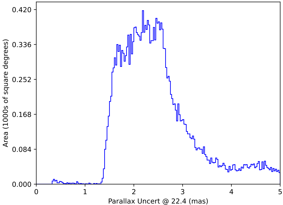
ddf_acor_sf10_lsf30_lsr10_v3.4_10yrs All sky: Parallax Uncert @ 22.4
