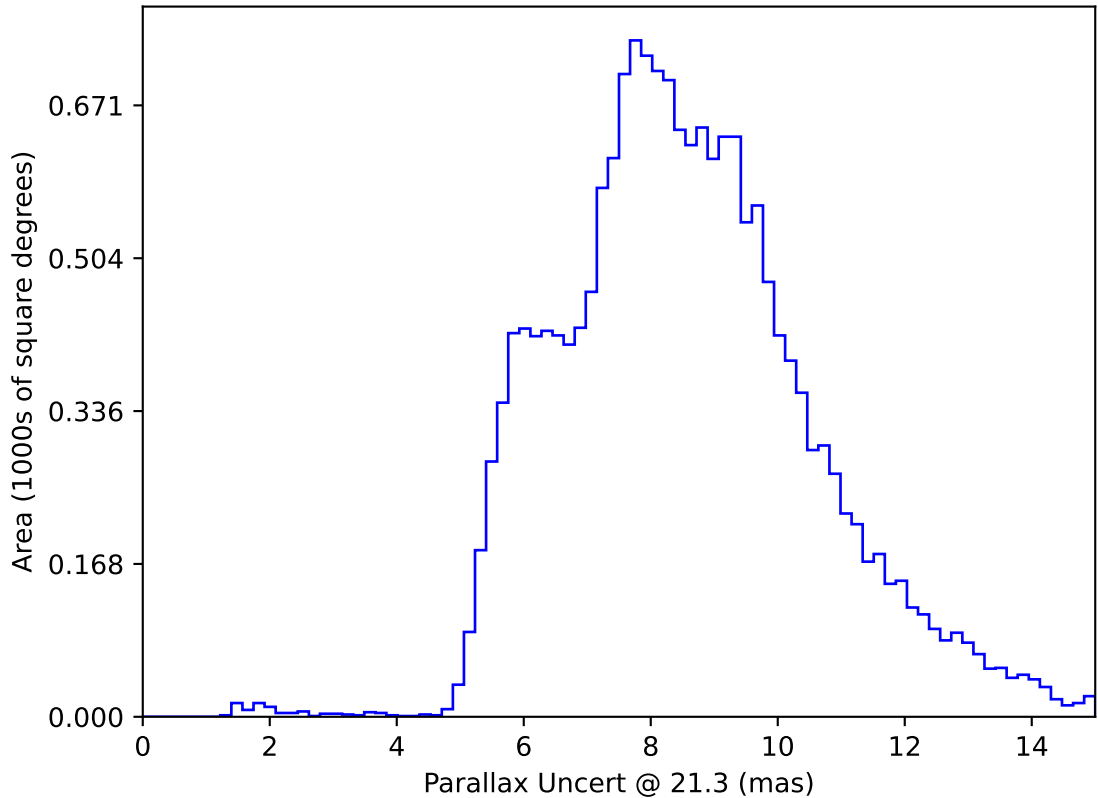
ddf_acor_sf10_lsf30_lsr10_v3.4_10yrs WFD y band only: Parallax Uncert @ 21.3
