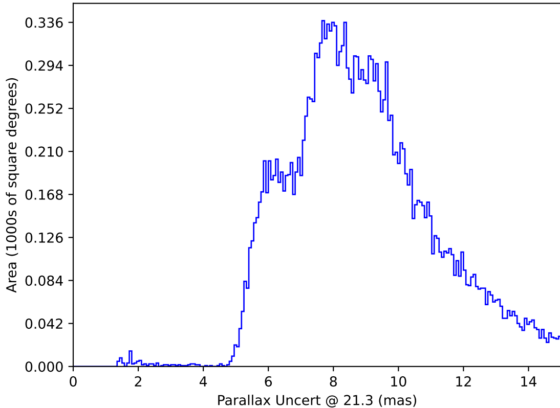
ddf_acor_sf10_lsf30_lsr10_v3.4_10yrs All sky y band only: Parallax Uncert @ 21.3
