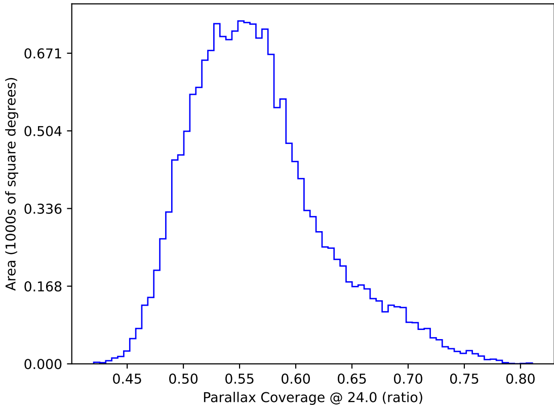
ddf_acor_sf10_lsf30_lsr10_v3.4_10yrs WFD: Parallax Coverage @ 24.0
