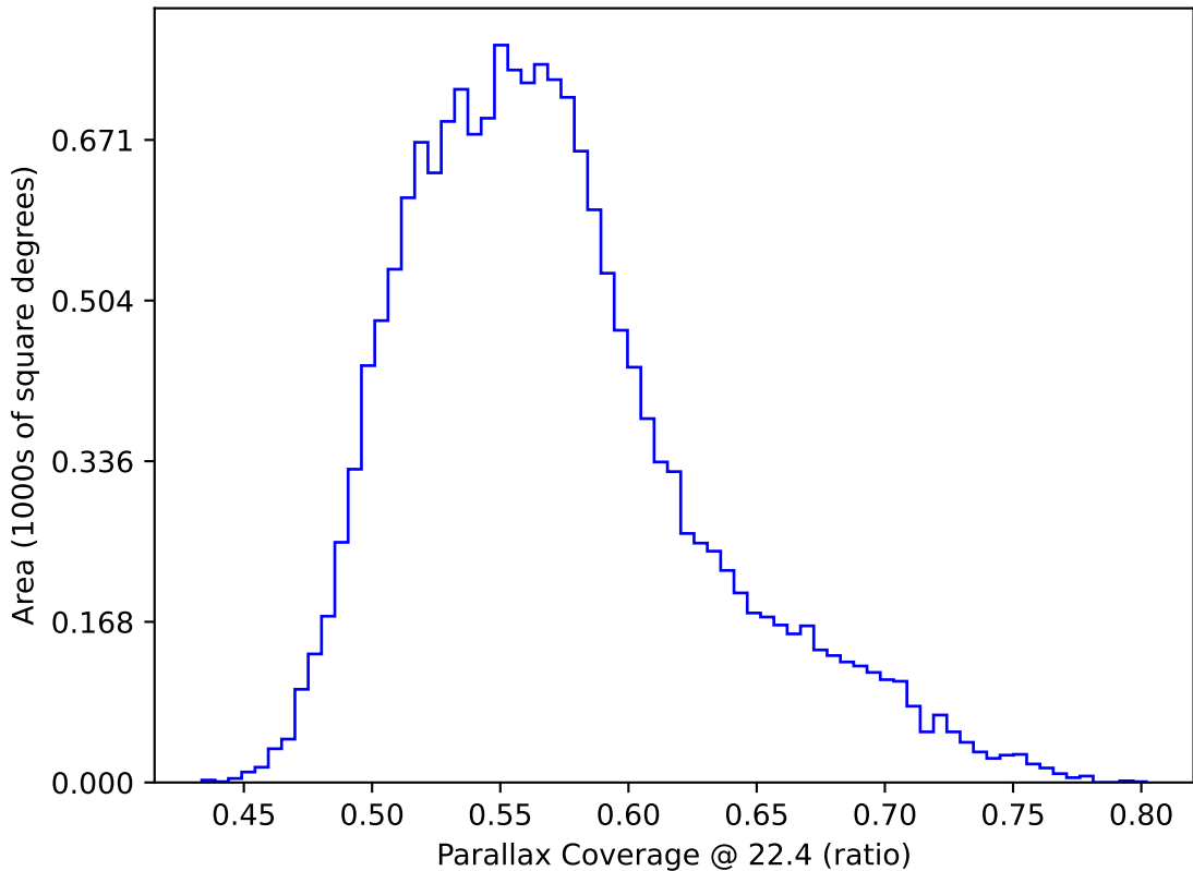
ddf_acor_sf10_lsf30_lsr10_v3.4_10yrs WFD: Parallax Coverage @ 22.4
