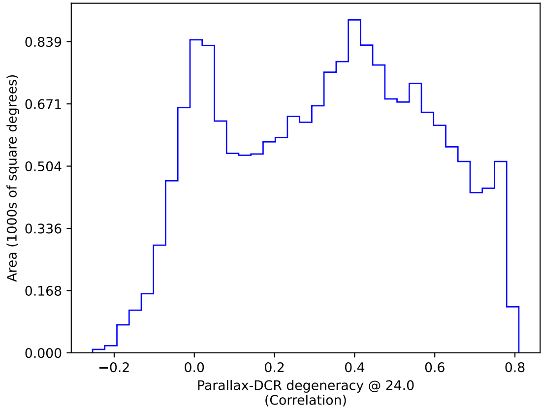
ddf_acor_sf10_lsf30_lsr10_v3.4_10yrs WFD: Parallax-DCR degeneracy @ 24.0
