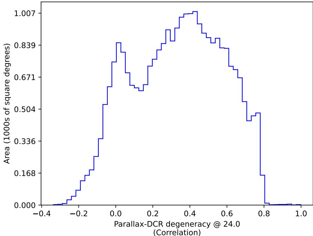
ddf_acor_sf10_ls30_lsr10_v3.4_10yrs All sky: Parallax-DCR degeneracy @ 24.0
