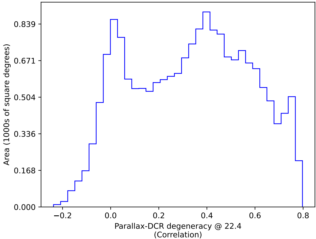
ddf_acor_sf10_lsf30_lsr10_v3.4_10yrs WFD: Parallax-DCR degeneracy @ 22.4
