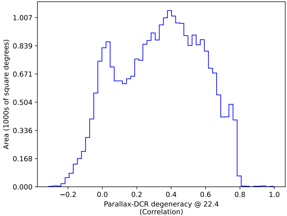
ddf_acor_sf10_ls30_lsr10_v3.4_10yrs All sky: Parallax-DCR degeneracy @ 22.4
