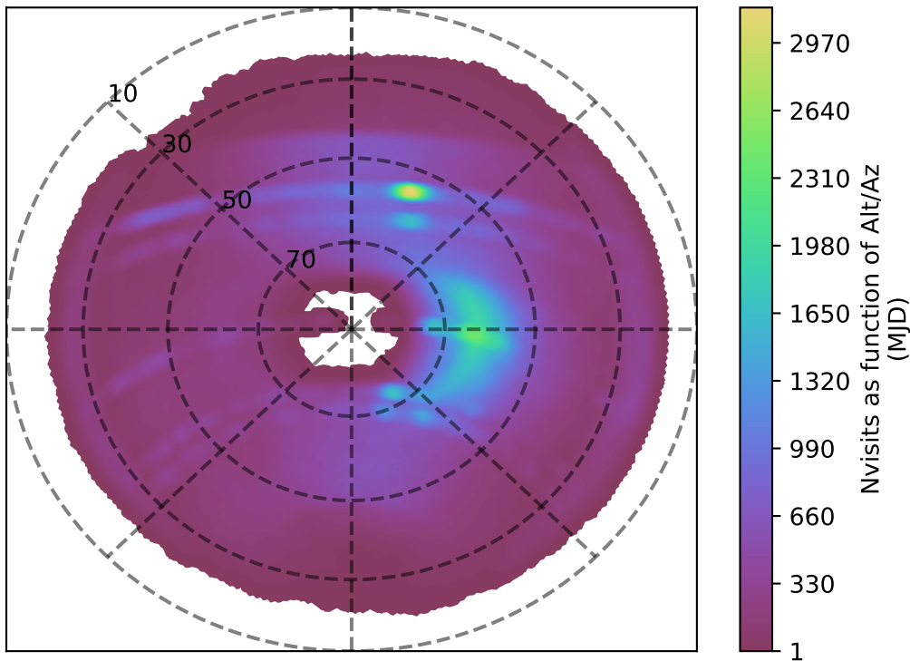
ddf_acor_sf10_lsf30_lsr10_v3.4_10yrs z band: Nvisits as function of Alt/Az
