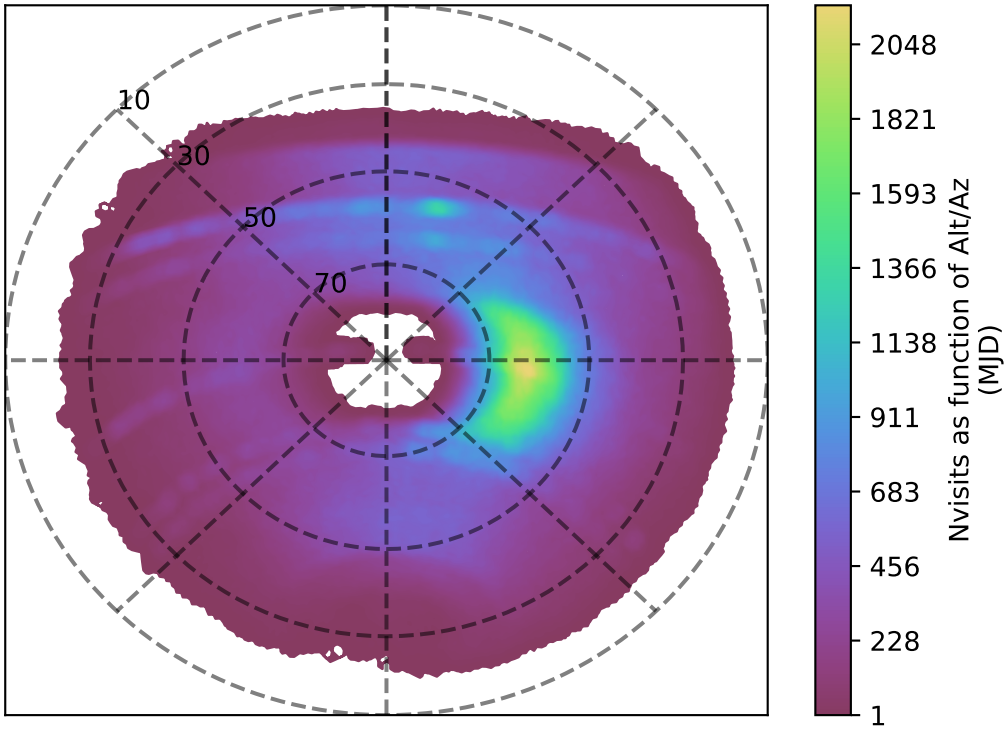
ddf_acor_sf10_lsf30_lsr10_v3.4_10yrs y band: Nvisits as function of Alt/Az
