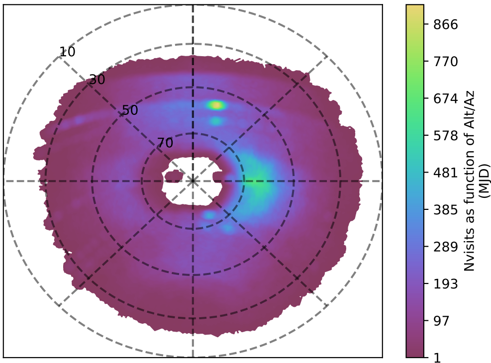
ddf_acor_sf10_lsf30_lsr10_v3.4_10yrs u band: Nvisits as function of Alt/Az
