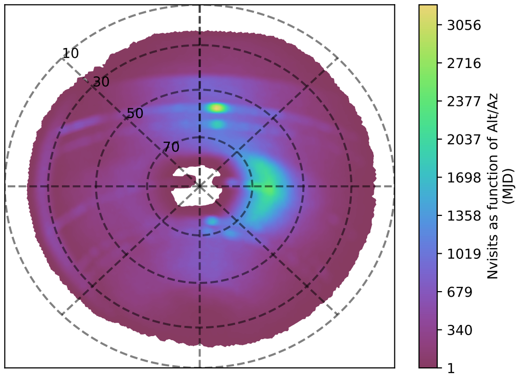
ddf_acor_sf10_lsf30_lsr10_v3.4_10yrs r band: Nvisits as function of Alt/Az
