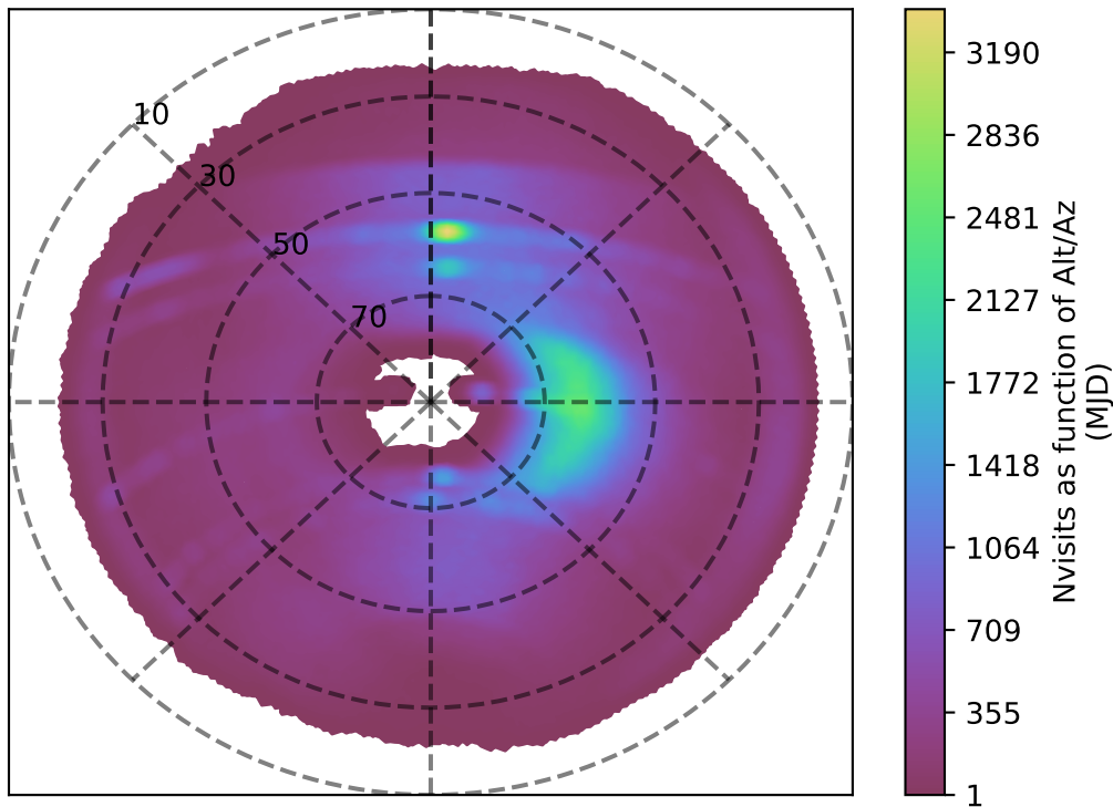
ddf_acor_sf10_lsf30_lsr10_v3.4_10yrs i band: Nvisits as function of Alt/Az
