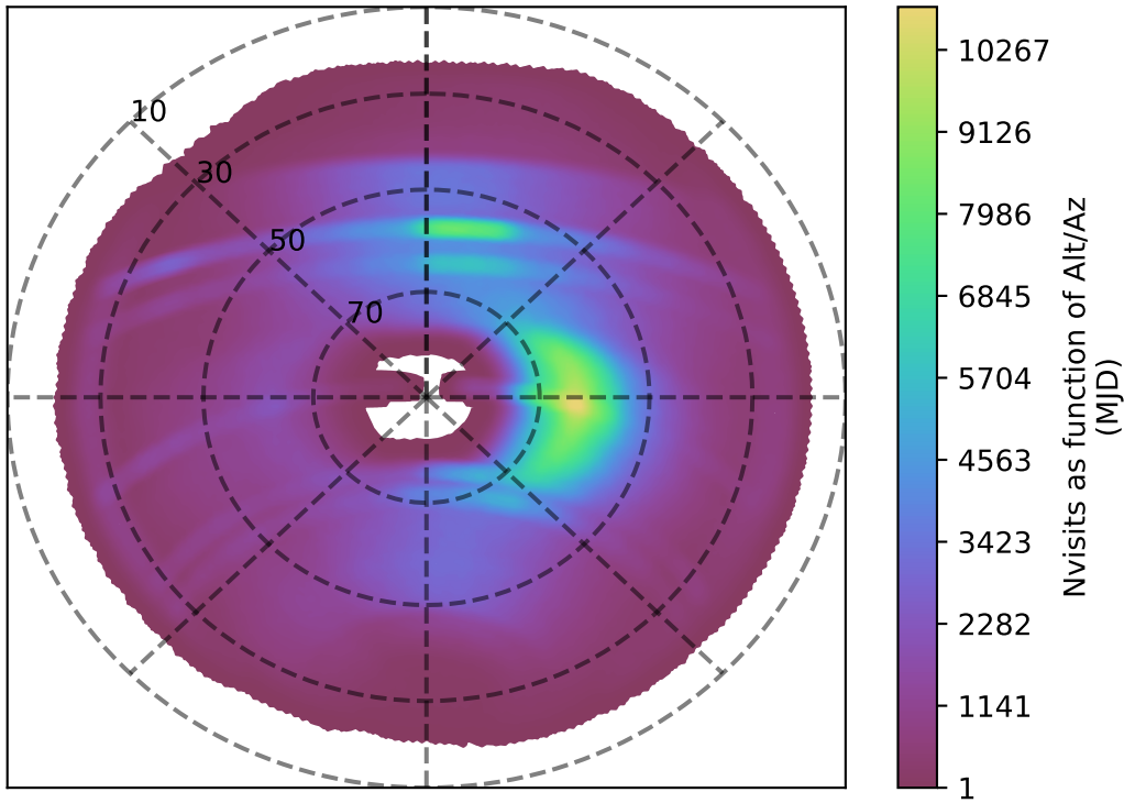
ddf_acor_sf10_ls30_lsr10_v3.4_10yrs all bands: Nvisits as function of Alt/Az
