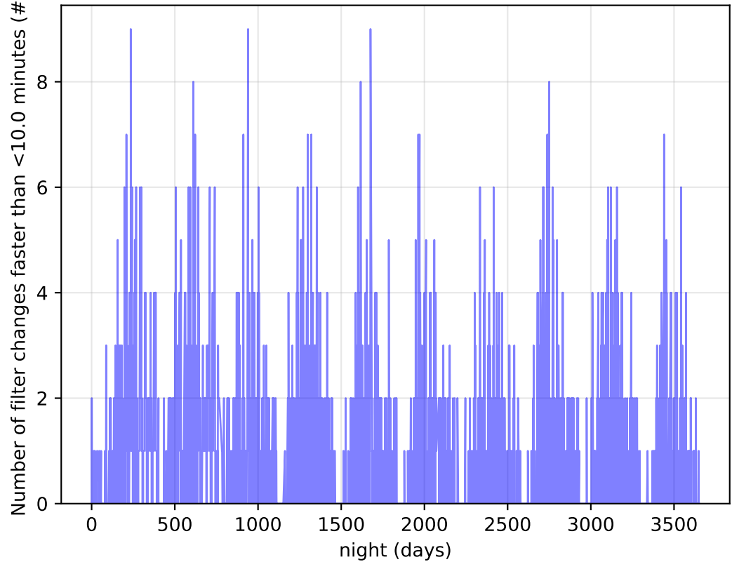
ddf_acor_sf10_Isf30_Isr10_v3.4_10yrs Per Night: Number of filter changes faster than <10.0 minutes
