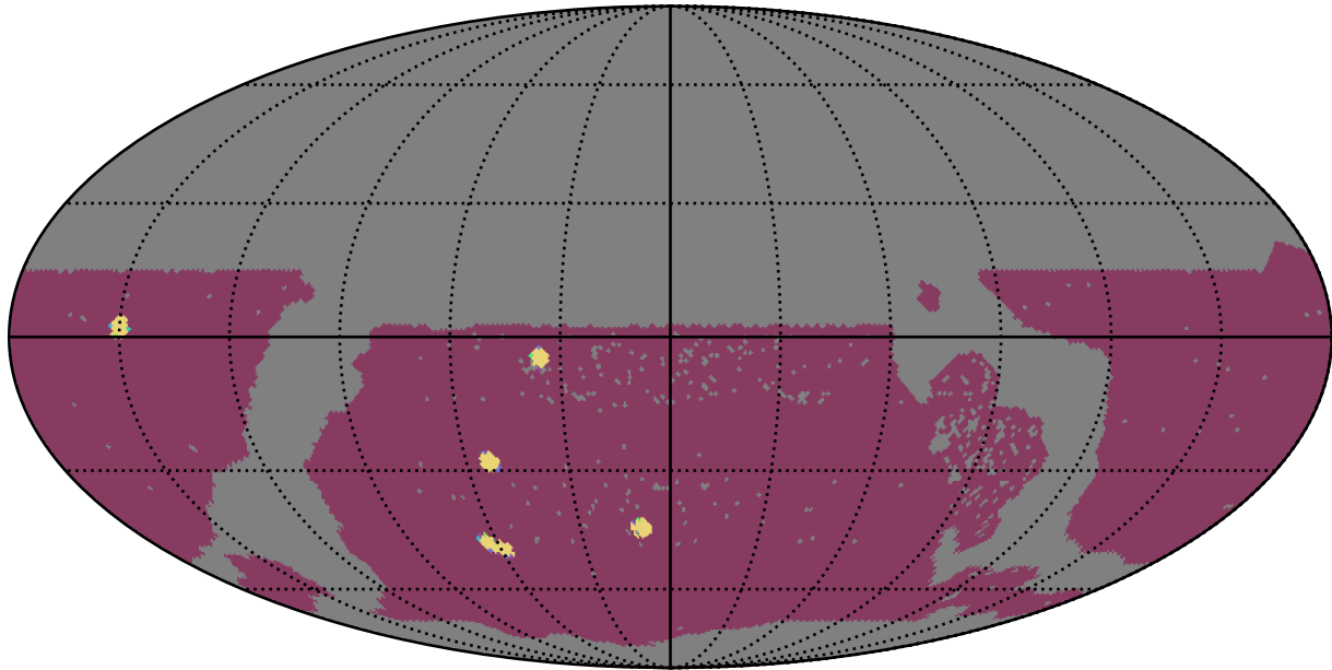
ddf_acor_sf10_lsf30_lsr10_v3.4_10yrs WFD: NumberOfQuickRevisits
