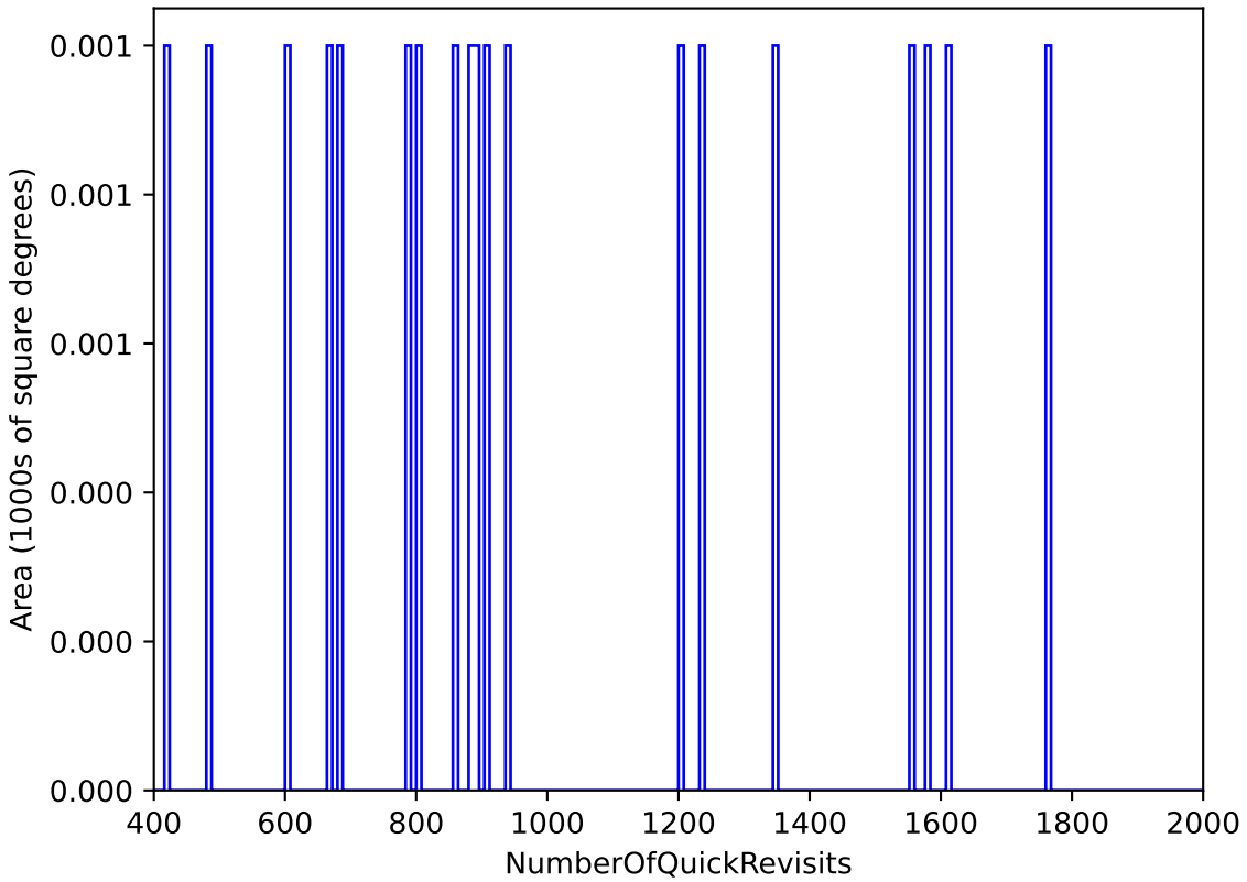
ddf_acor_sf10_lsf30_lsr10_v3.4_10yrs WFD: NumberOfQuickRevisits
