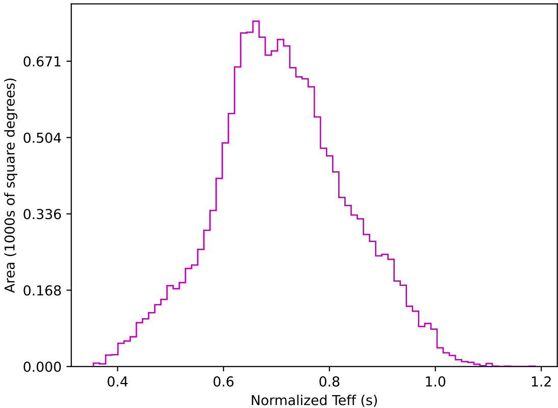
ddf_acor_sf10_lsf30_lsr10_v3.4_10yrs WFD z band: Normalized Teff
