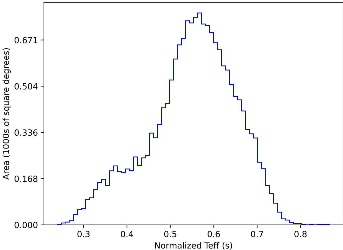
ddf_acor_sf10_lsf30_lsr10_v3.4_10yrs WFD y band: Normalized Teff
