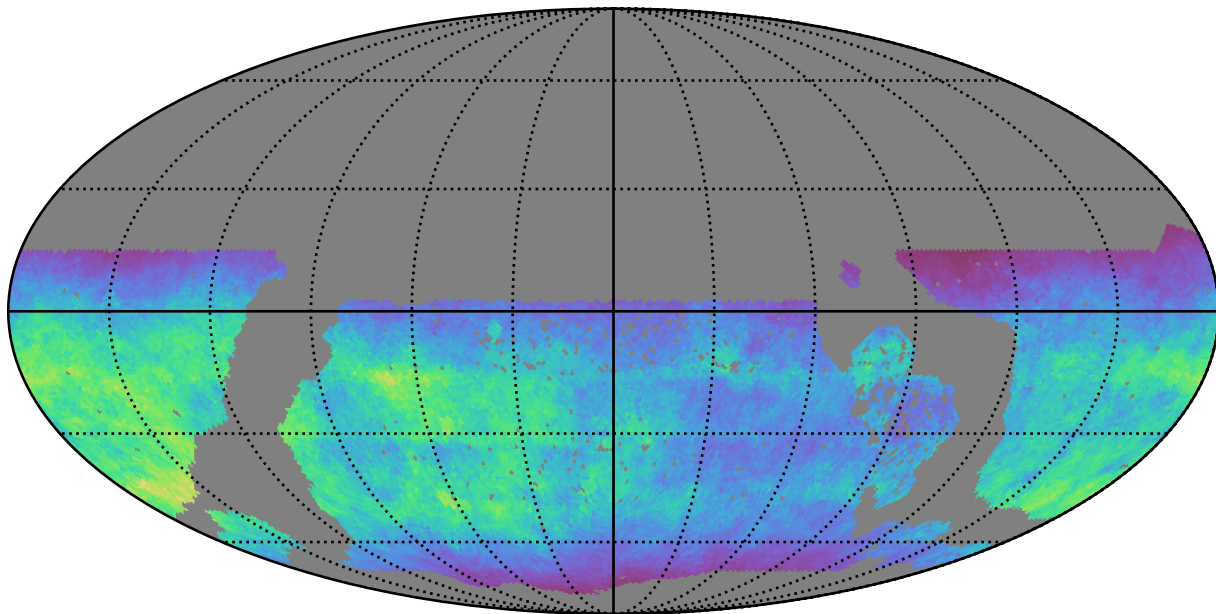
ddf_acor_sf10_lsf30_lsr10_v3.4_10yrs WFD u band: Normalized Teff
