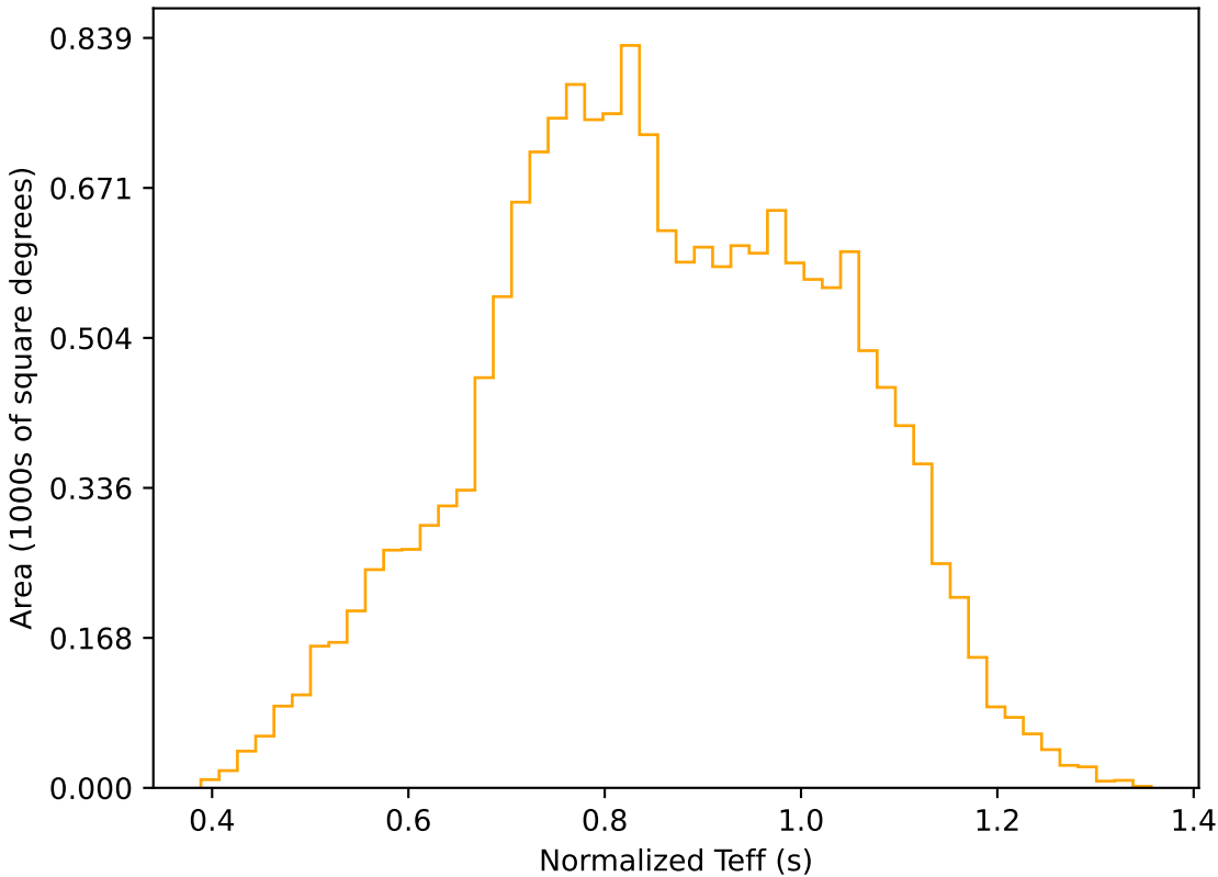
ddf_acor_sf10_lsf30_lsr10_v3.4_10yrs WFD r band: Normalized Teff
