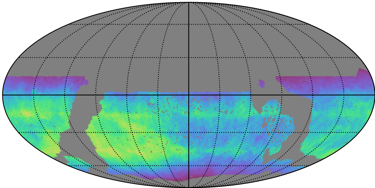
ddf_acor_sf10_lsf30_lsr10_v3.4_10yrs WFD i band: Normalized Teff
