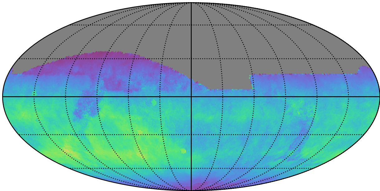
ddf_acor_sf10_lsf30_lsr10_v3.4_10yrs All sky z band: Normalized Teff
